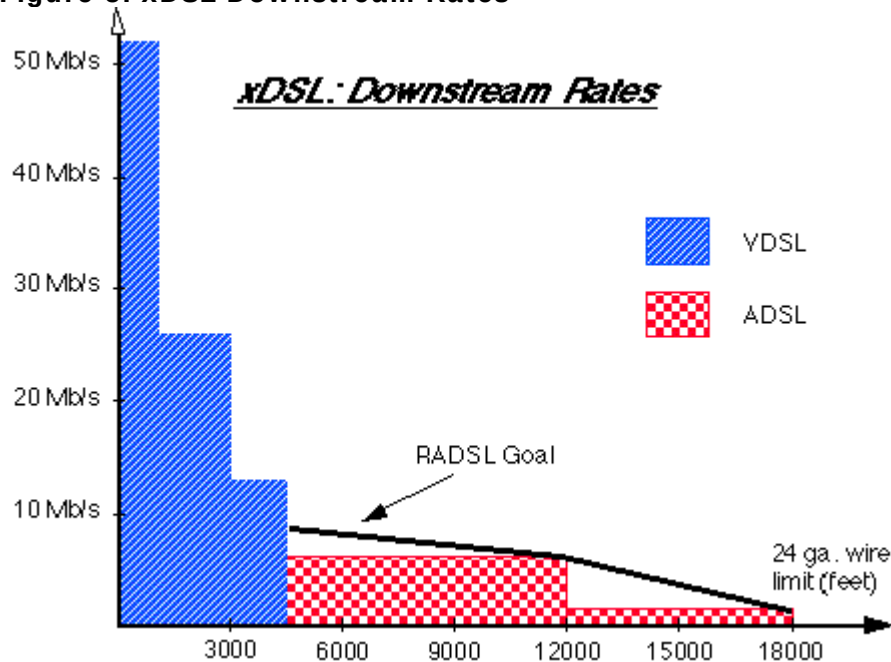
Figure 5. xDSL Downstream Rates
