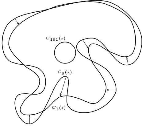
Figure 3: C_1(s) and C_{101}(s) obtained from geometric evolution of the closed simple curve C_0(s) .
