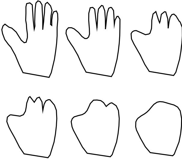
Figure 4: Geometric evolution of a closed simple curve.
