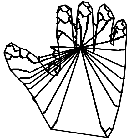
Figure 5: Geometric evolution paths of some points on the curve of Fig. 4.
