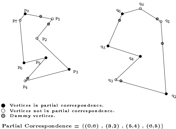
Figure 6: Completing a partial correspondence to a full correspondence: Given polygon P with 8 vertices, Q with 7 vertices and a partial correspondence of 4 pairs, the partial correspondence is completed to 11 pairs by adding 3 dummy vertices to P , and 4 to Q .
