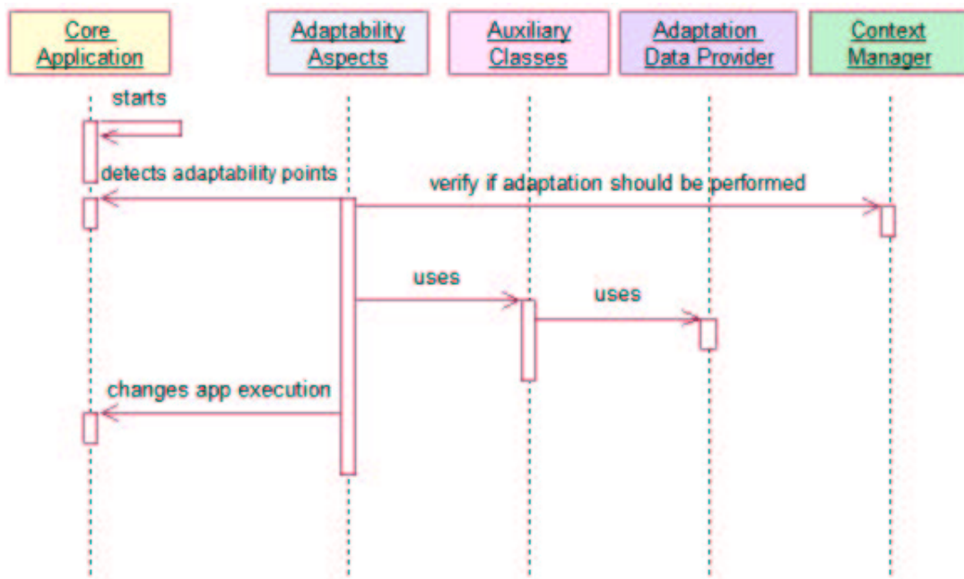
Figure 2: Dynamics of AdapPE pattern (scenario I)
