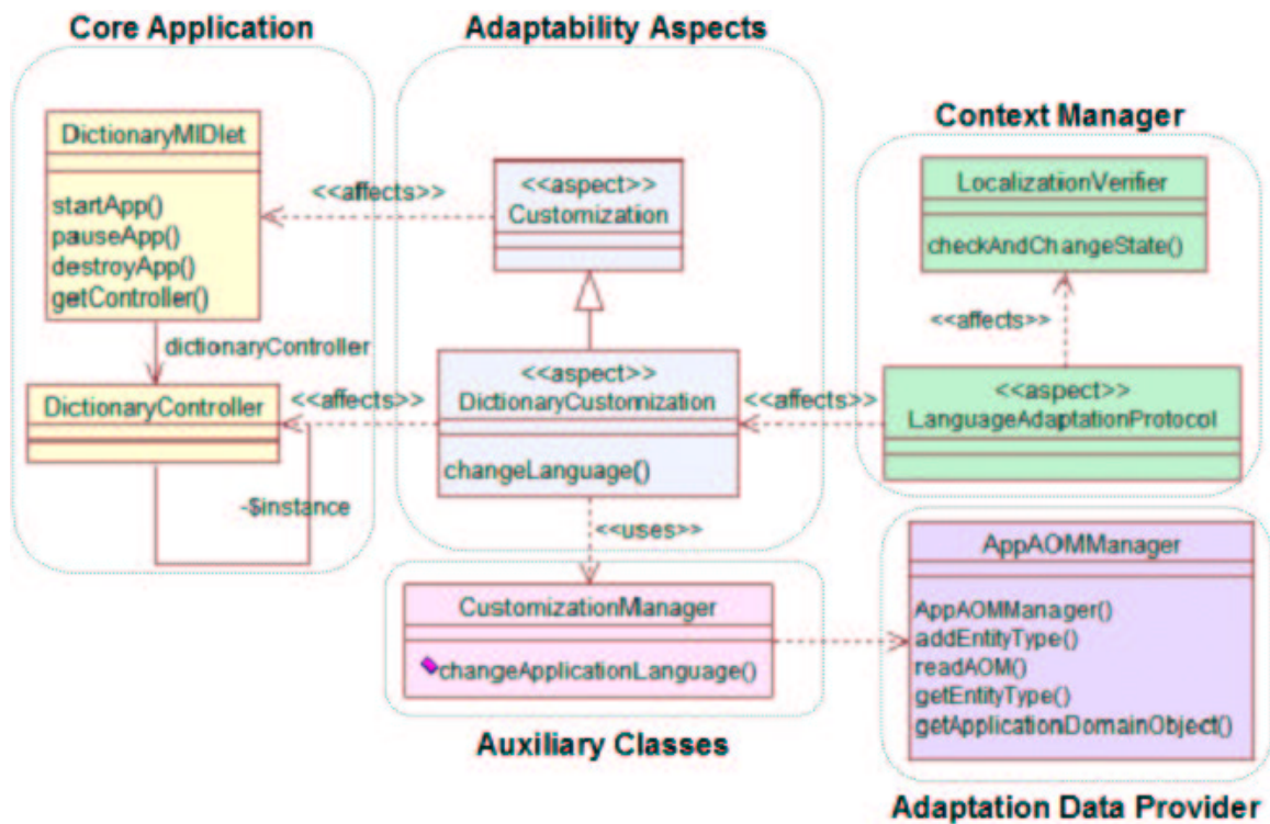
Figure 7: An AdapPE pattern example
