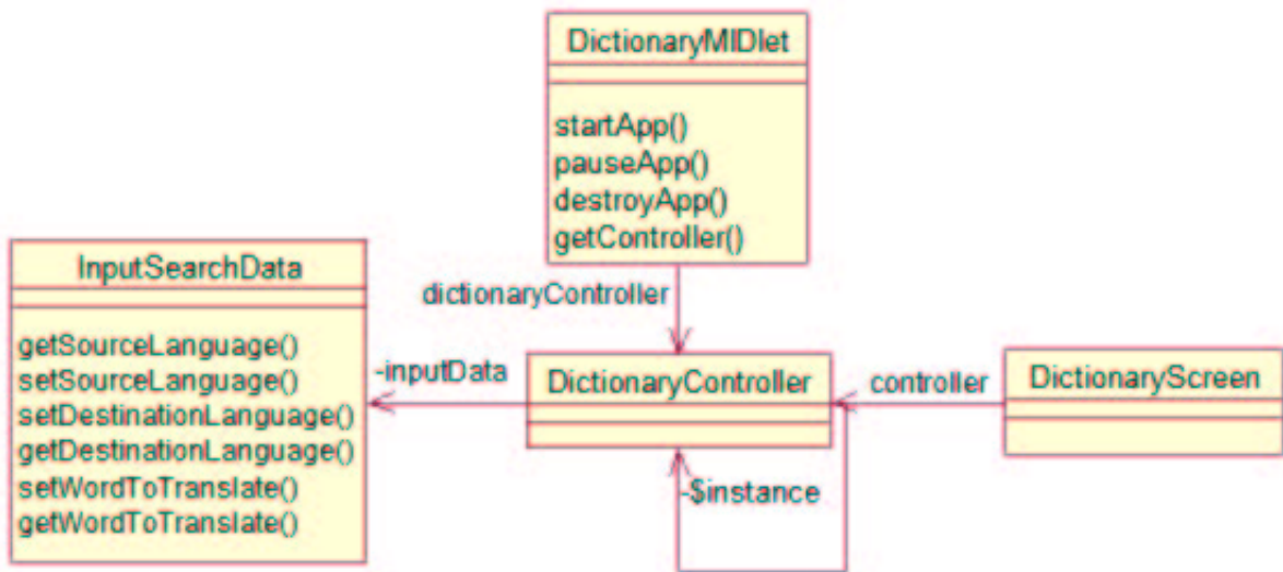
Figure 6: A Core Application example
