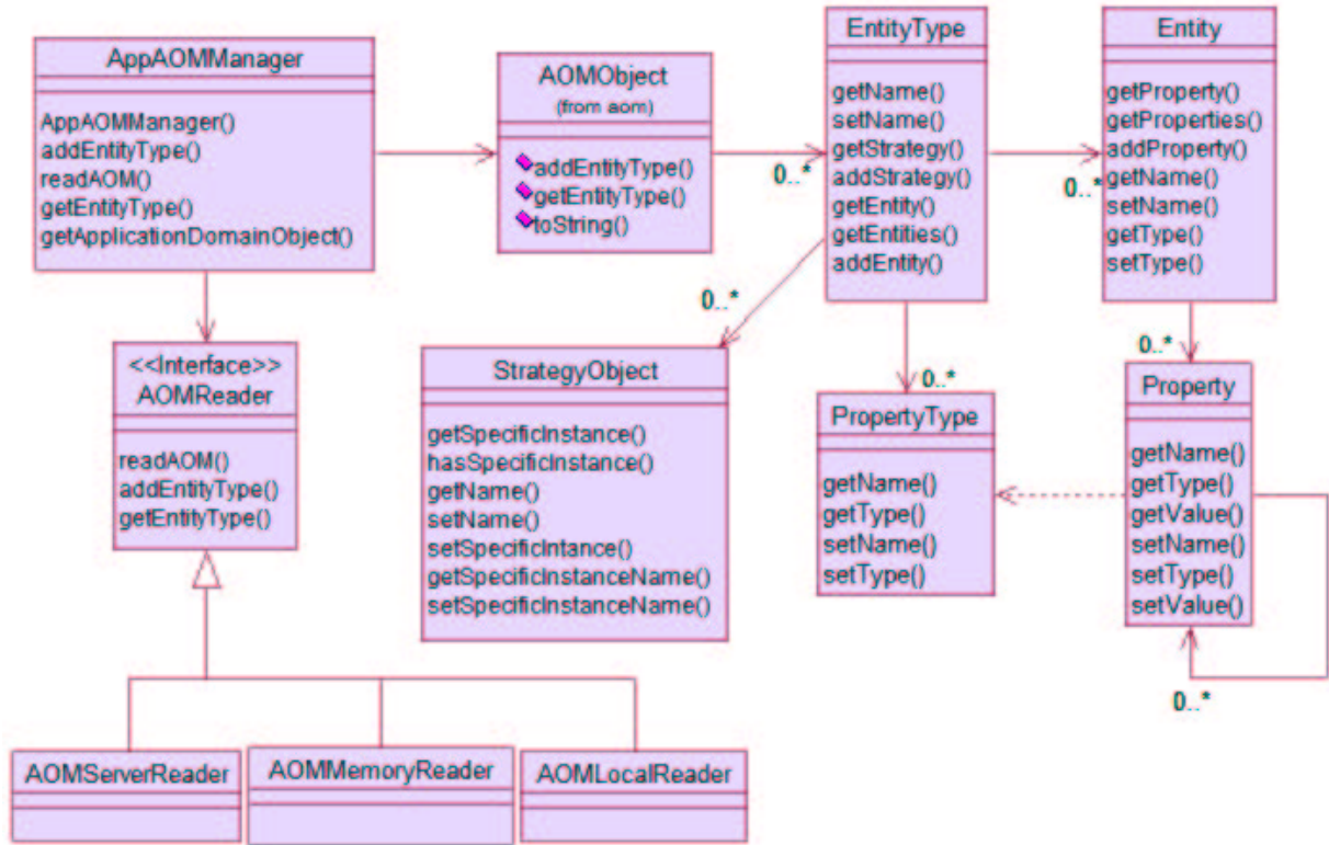
Figure 5: Adaptation Data Provider using AOM
