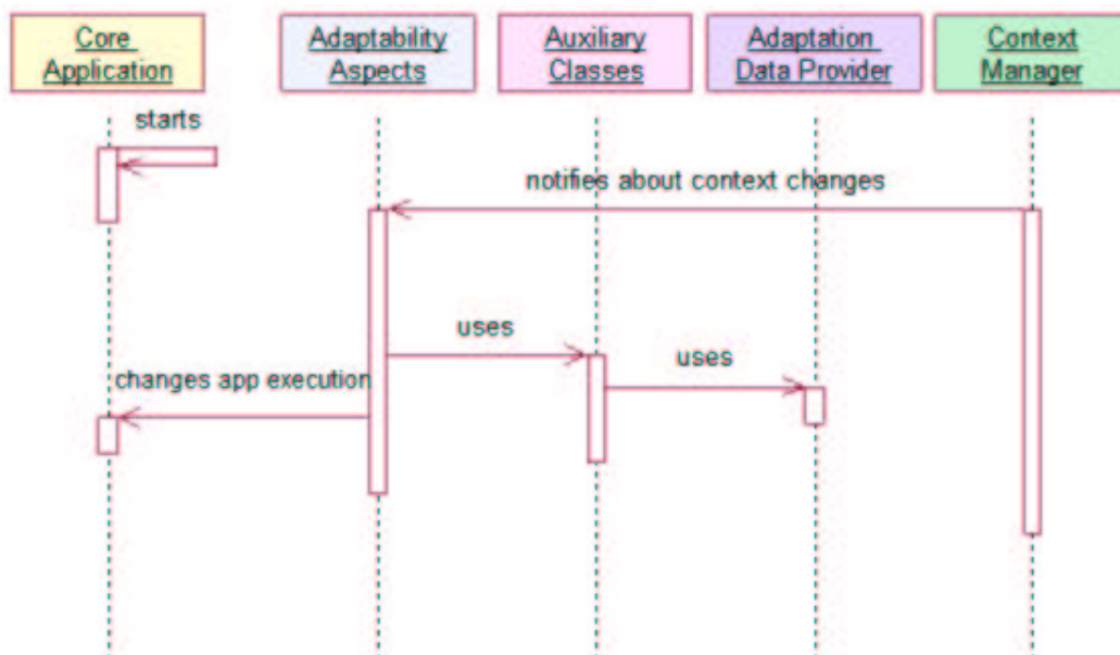
Figure 3: Dynamics of the AdapPE pattern (scenario II)
