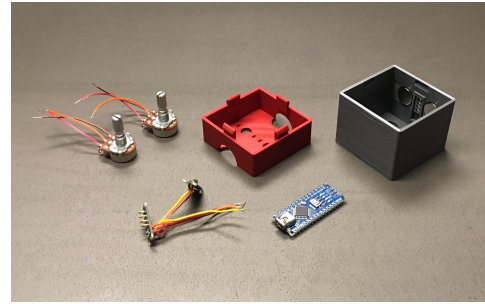
Figure 4: Example of an open block showing sensors (two pots), microcontroller, and pogo-pcb with pogo pins.
