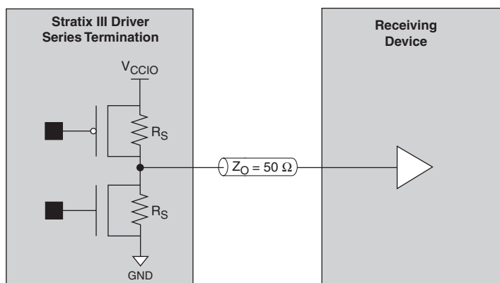
Figure 7-9. Stratix III On-Chip Series Termination without Calibration
