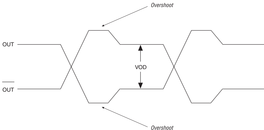
Figure 9–10. Programmable VOD
