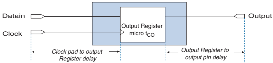
Figure 1–3. Output Register Clock to Output Timing Diagram
