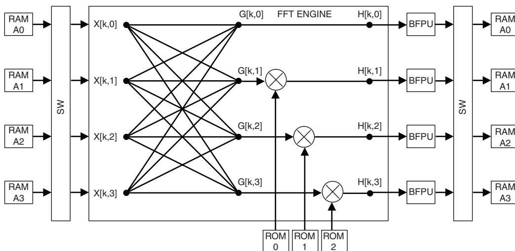
Figure 5–24. Radix-4 Butterfly
