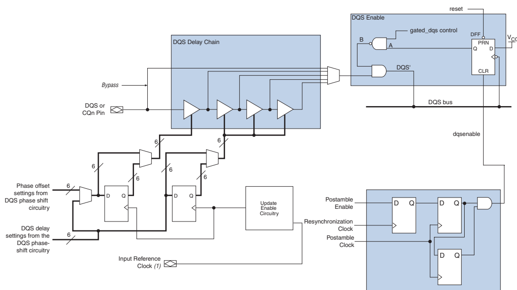
Figure 8–13. Stratix III DQS Logic Block
