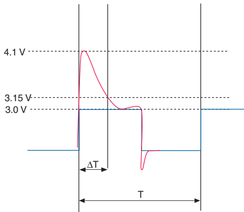
Figure 1–1. Overshoot Duration
