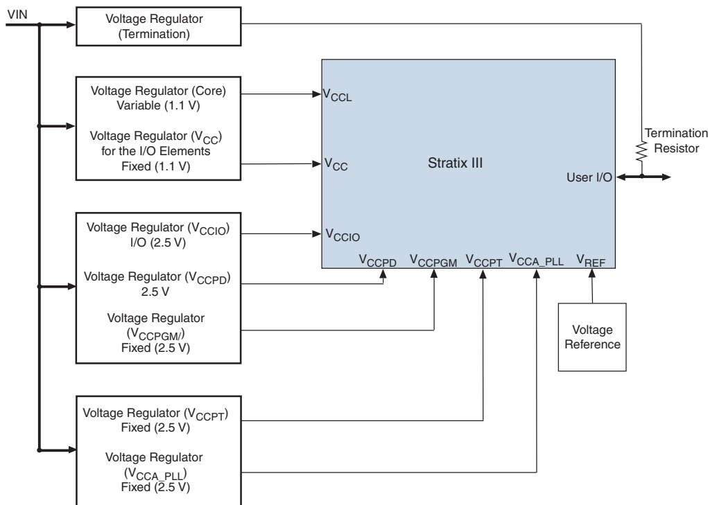
Figure 16–1. Stratix III Power Management Example
