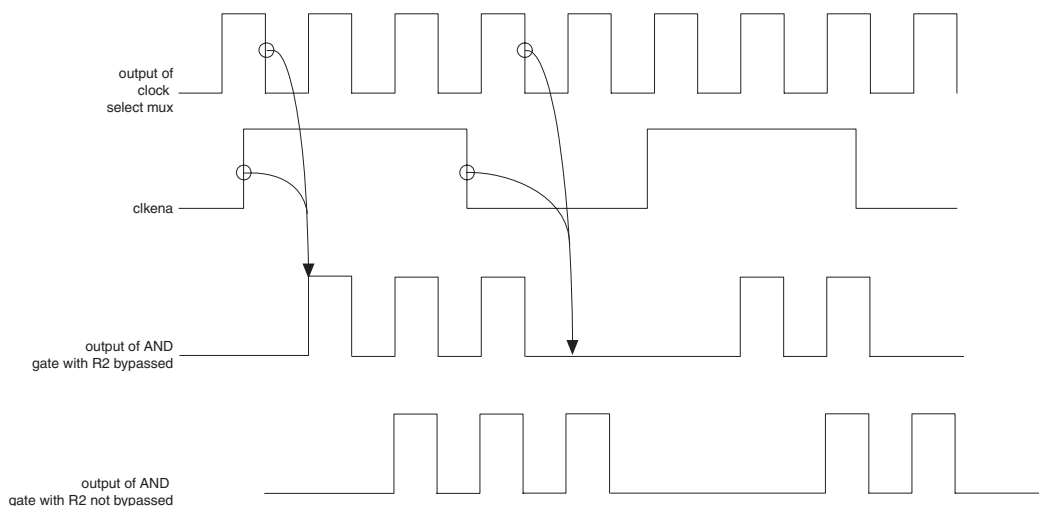
Figure 6–15. clkena Signals
