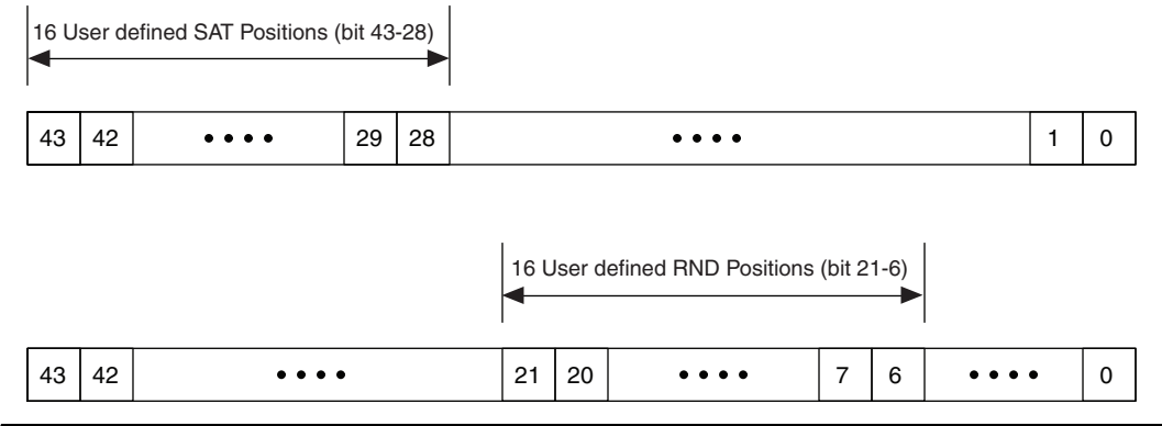
Figure 5–20. Round and Saturation Locations
