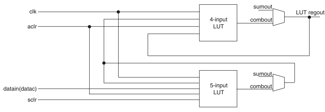
Figure 2–15. LUT Register from Two Combinational Blocks
