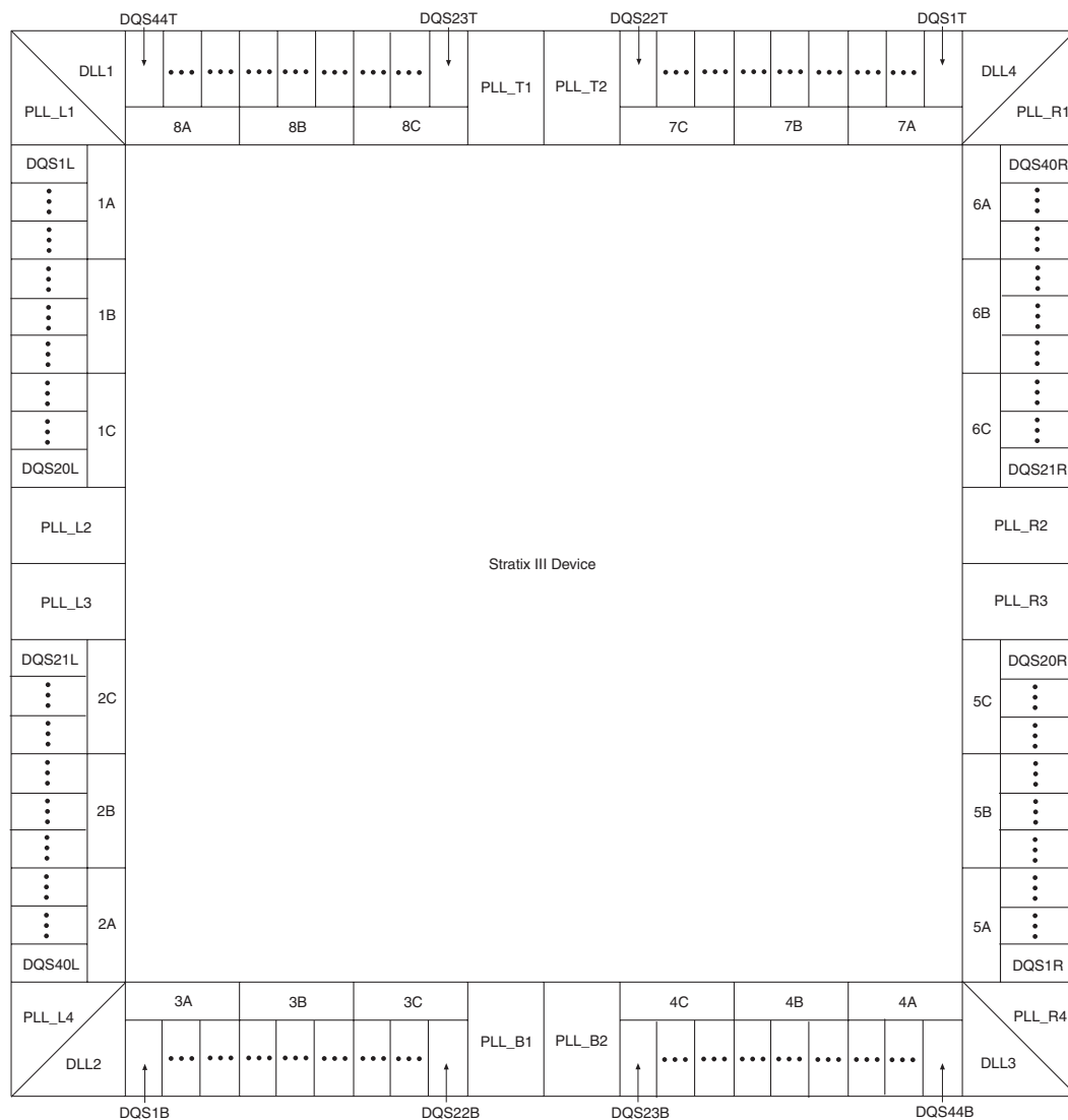
Figure 8–8. DQS Pins in Stratix III I/O Banks
