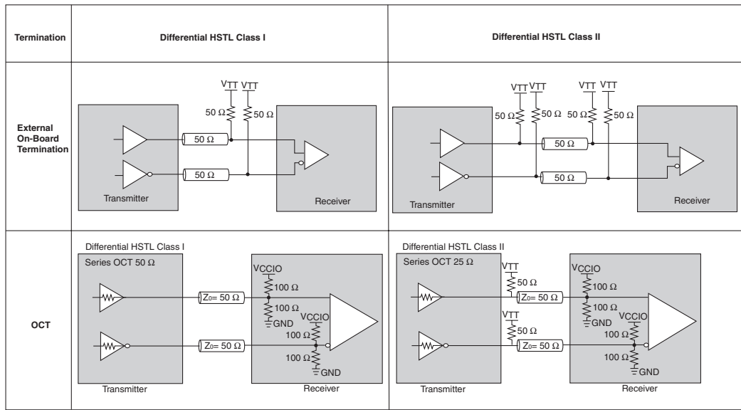
Figure 7–24. Stratix III Differential HSTL I/O Standard Termination
