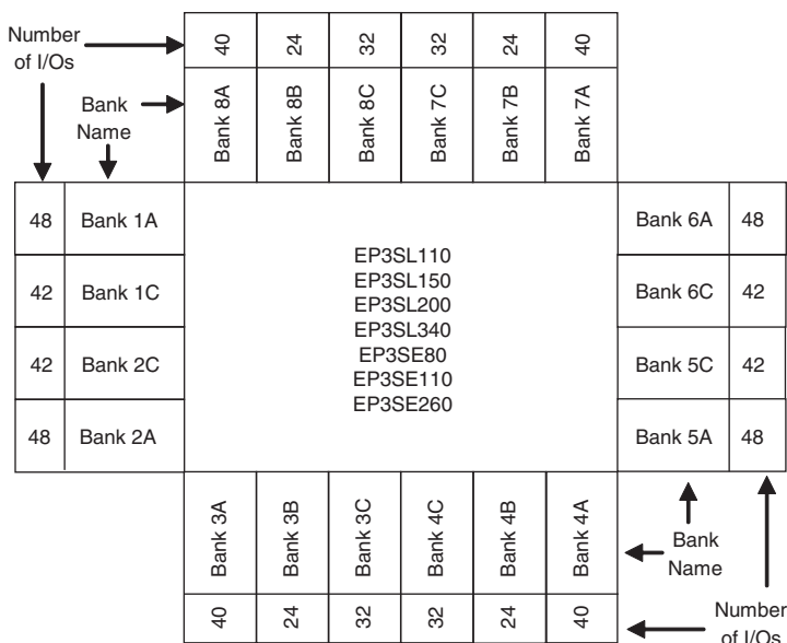
Figure 7–5. Number of I/Os in Each Bank in EP3SL110, EP3SL150, EP3SL200, EP3SE80, EP3SE110 and EP3SE260 Devices in the 1152-pin FineLine BGA Package. Number of I/Os in Each Bank in EP3SL340 in the 1152-pin Hybrid FineLine BGA Package Note (1), (2)
