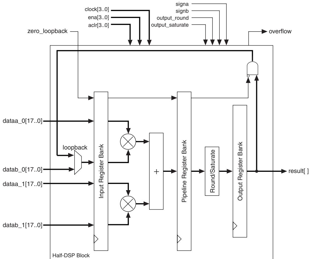
Figure 5–15. Loopback Mode for Half-DSP Block
