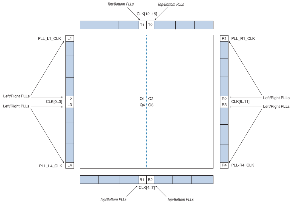
Figure 6–16. Stratix III PLL Locations
