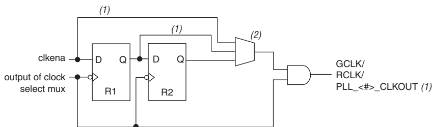
Figure 6–14. clkena Implementation
