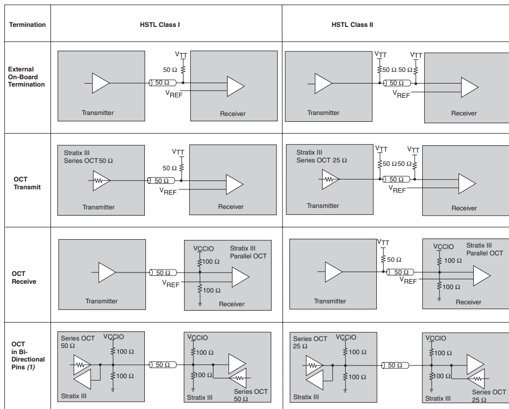
Figure 7–22. Stratix III HSTL I/O Standard Termination
