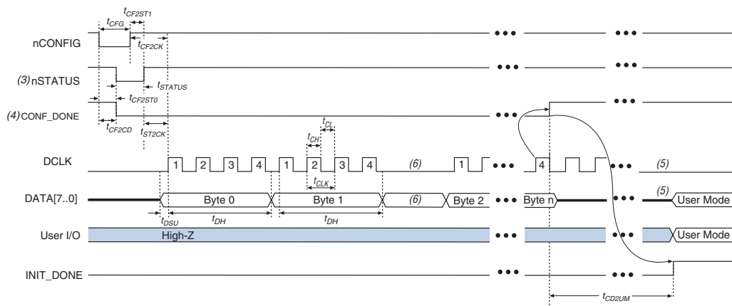
Figure 11–7. FPP Configuration Timing Waveform With Decompression or Design Security Feature Enabled Notes (1), (2)
