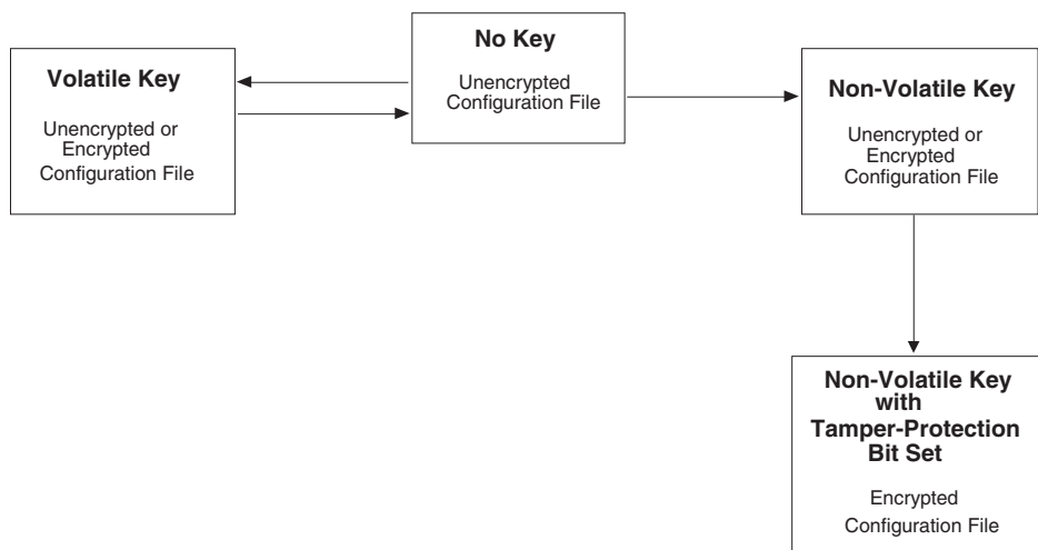
Figure 14–2. Stratix III Security Modes - Sequence and Restrictions
