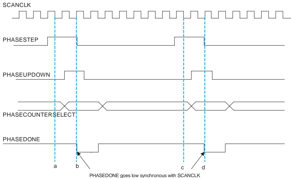
Figure 6–41. Dynamic Phase Shifting Waveform
