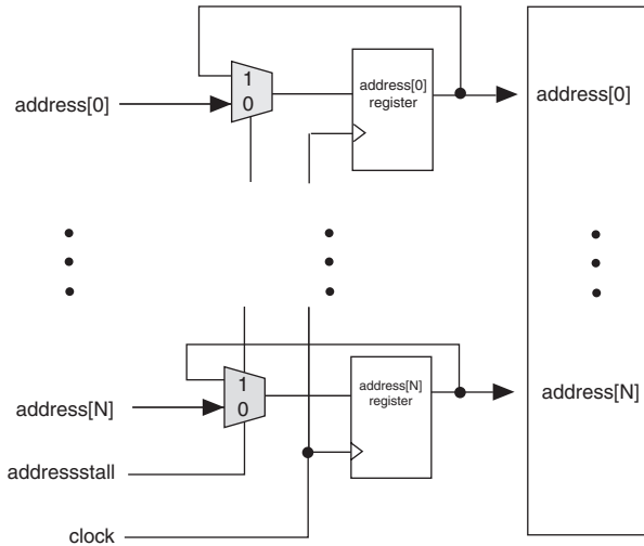
Figure 4–2. Stratix III Address Clock Enable Block Diagram
