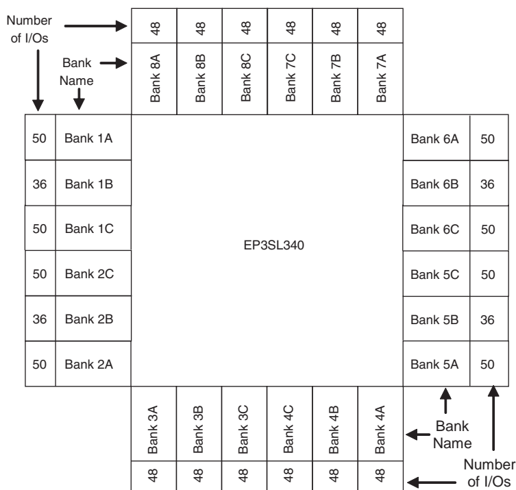
Figure 7–7. Number of I/Os in Each Bank in EP3SL340 Devices in the 1760-pin FineLine BGA Package
