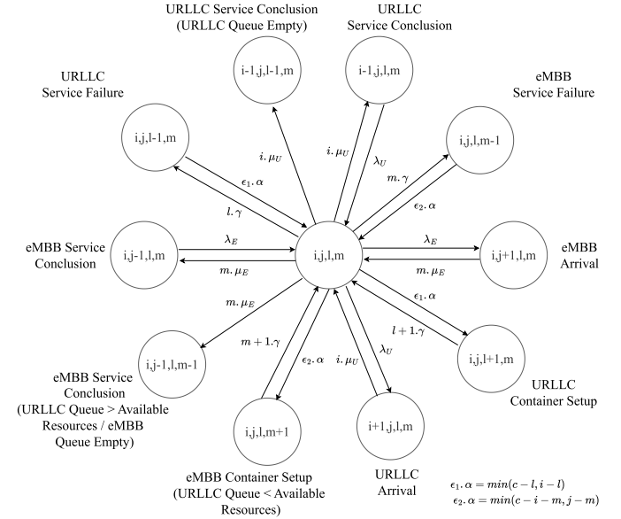
Fig. 1. Generic CTMC State Diagram
