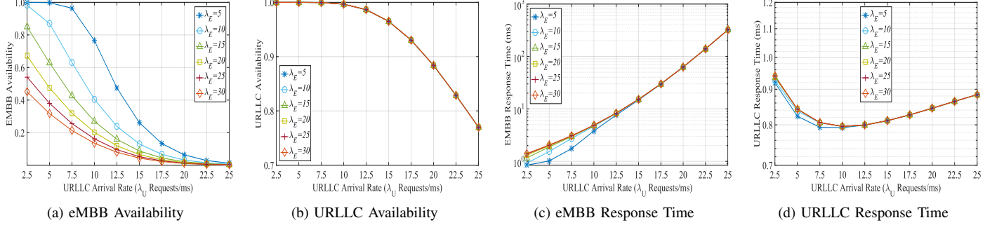
Fig. 2. Effects of the eMBB load ( \lambda_E )
