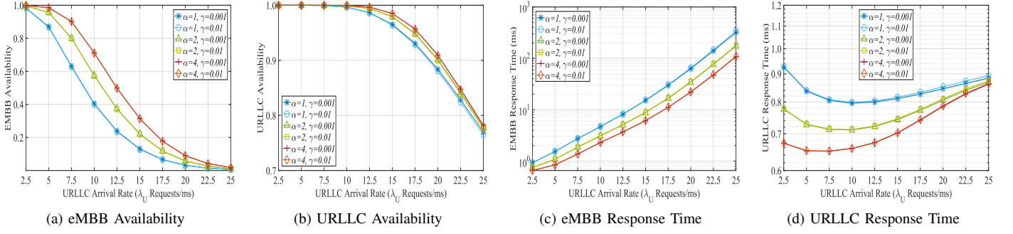
Fig. 3. Effects of the container setup rate ( \alpha ) and service failure rate ( \gamma )
