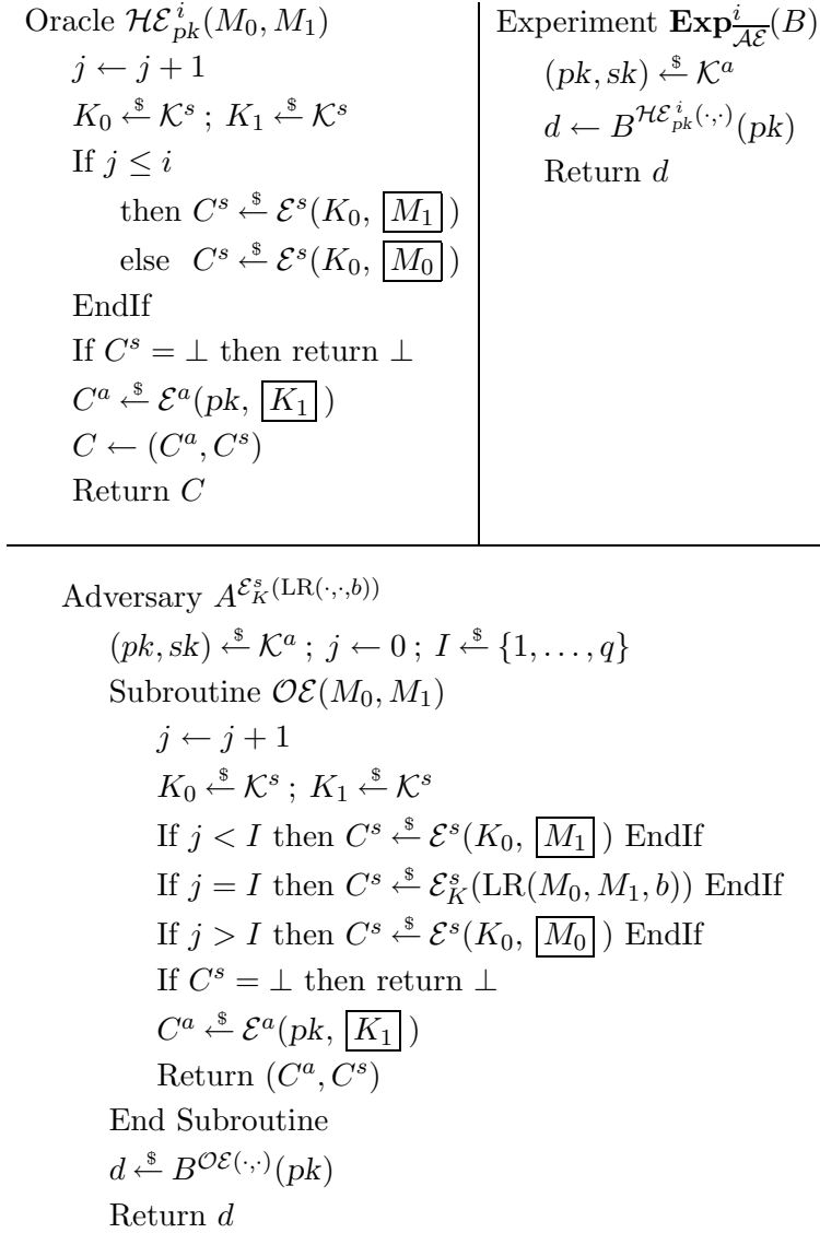
Figure 11.4: Hybrid oracles and experiments related to the construction of ind-cpa adversary A in the proof of Theorem 11.6.
