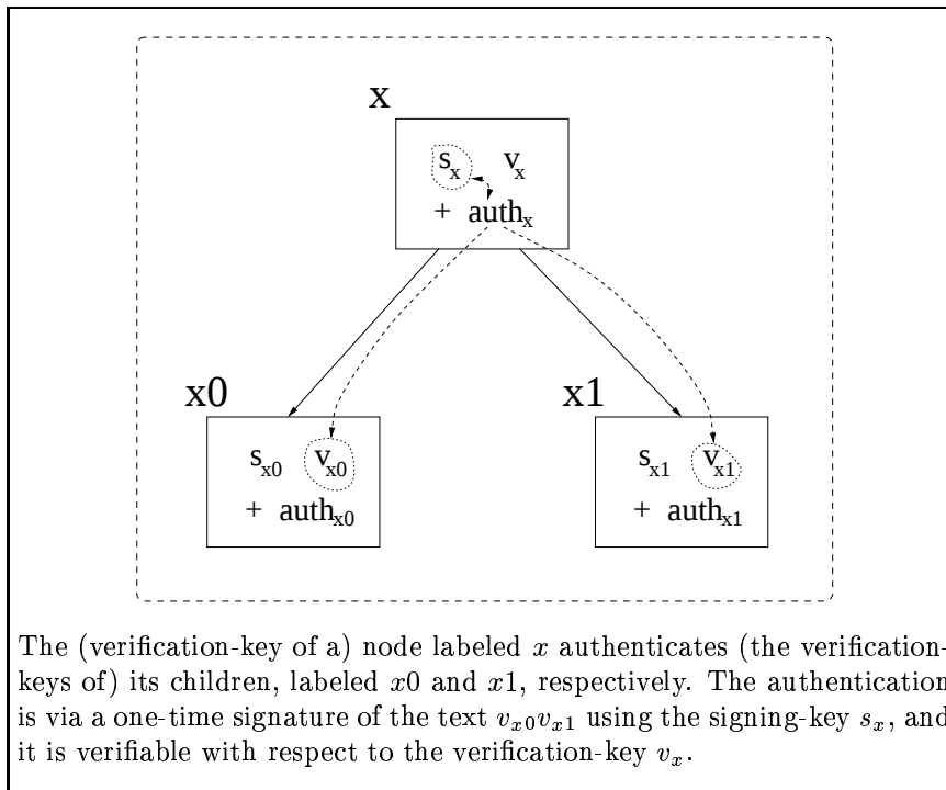
Figure 6.2: Authentication trees: the basic authentication step.
