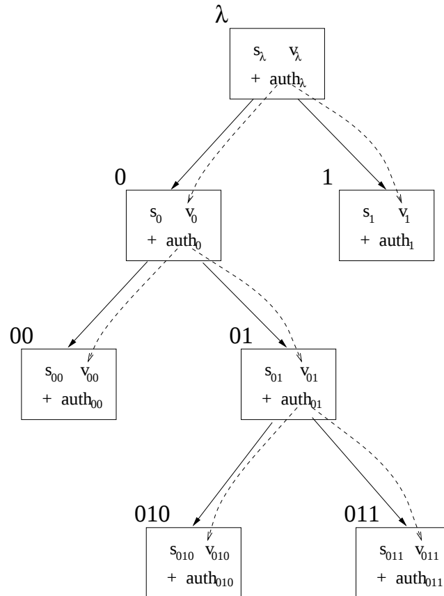
Figure 6.3: An authentication path for nodes 010 and 011.
